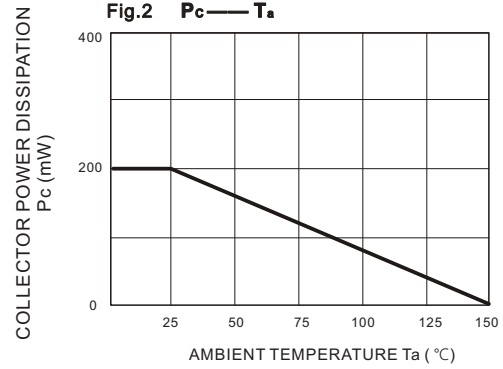
Fig.2 P_c — T_a
