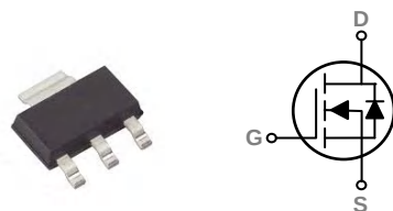
SOT223 Pin Configuration
