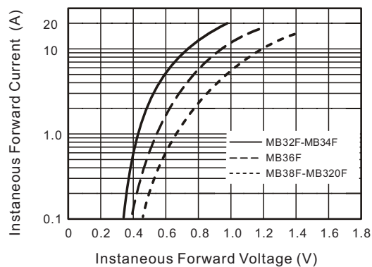
FIG.2-TYPICAL FORWARD CHARACTERISTICS
