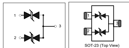
Schematic & PIN Configuration
